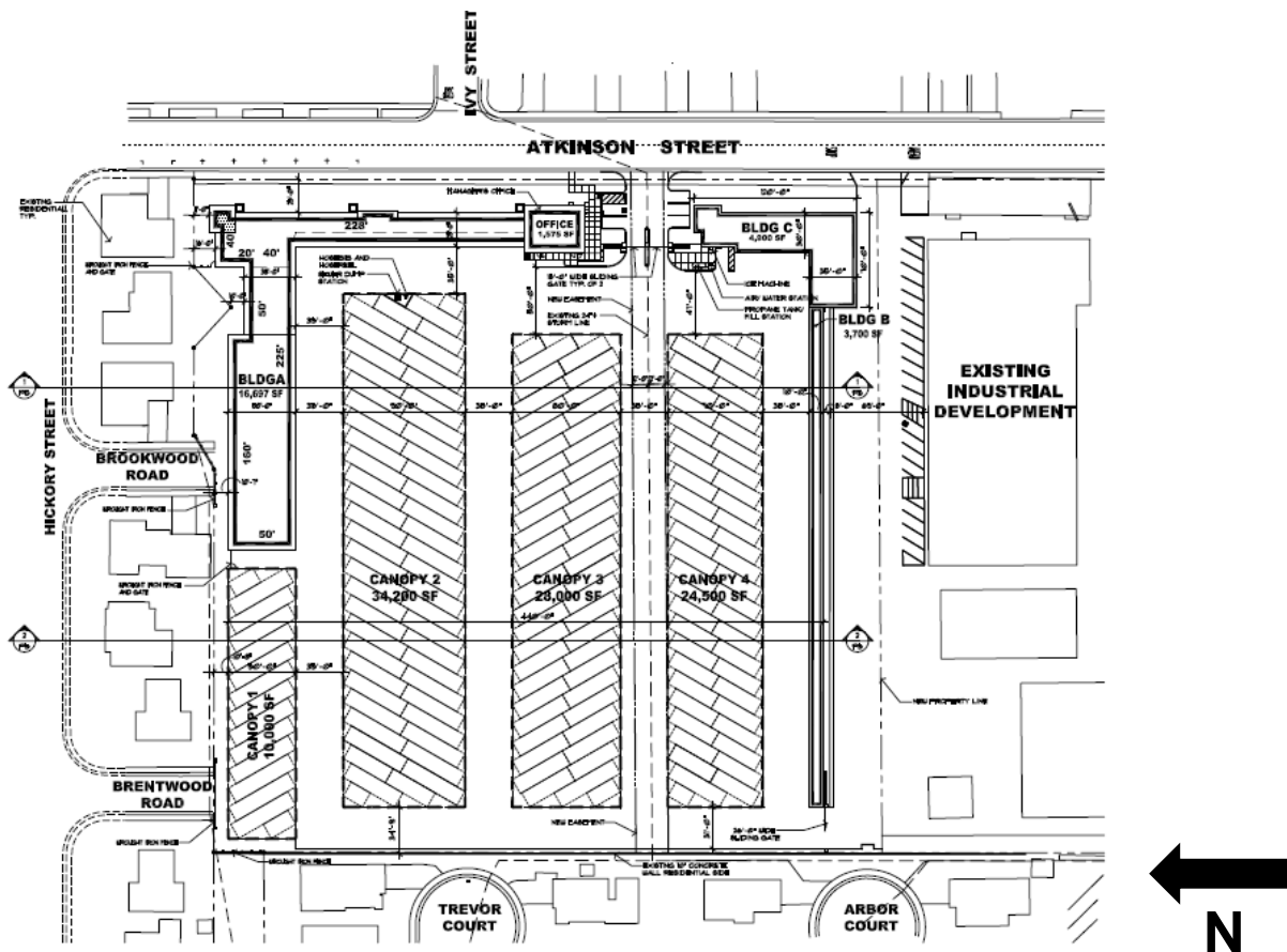
Figure 2. Site Plan
